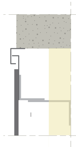
Figure 21: EQUITONE to render side abutment
